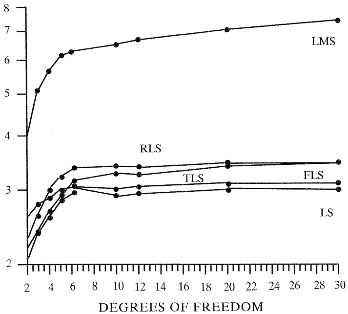
Figure 4. IO-scheme: Efficiency under Student's-t errors
