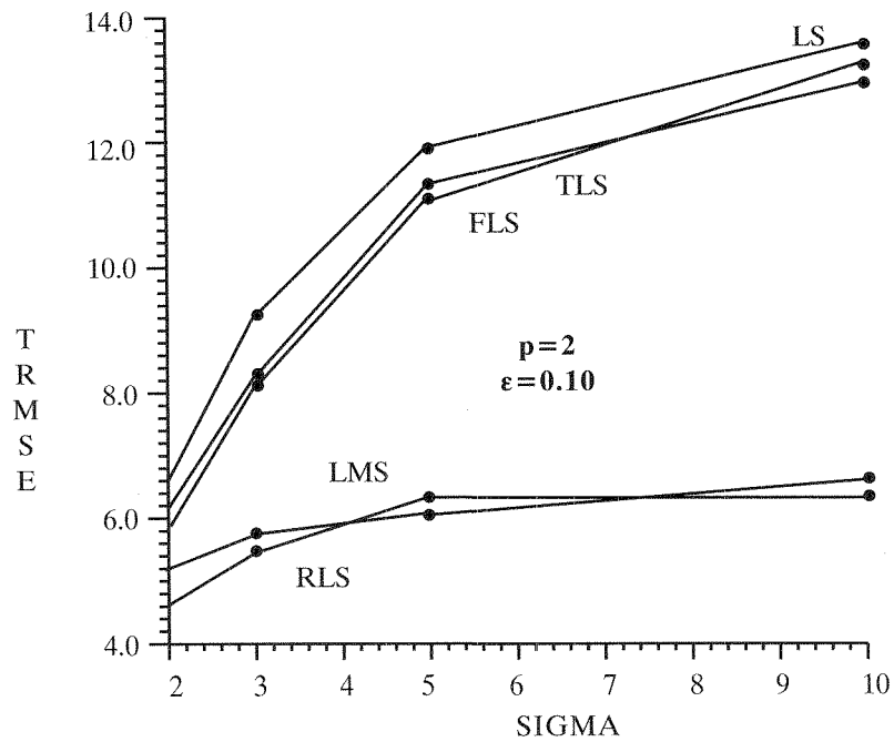
Figure 8. AO-scheme: Efficiency under normal additive effects
