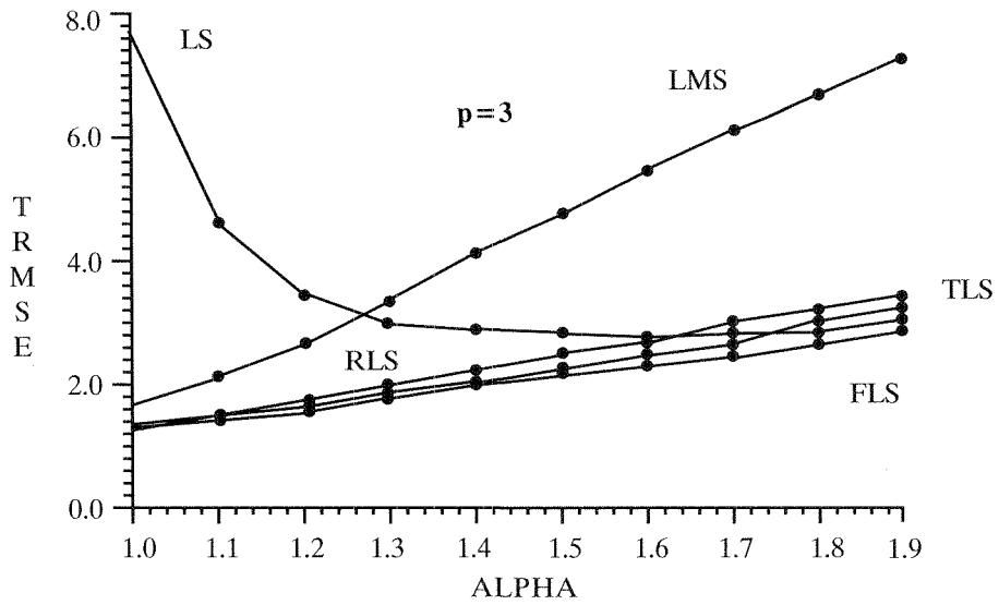
Figure 1. IO-scheme: Efficiency under symmetric-samle errors
