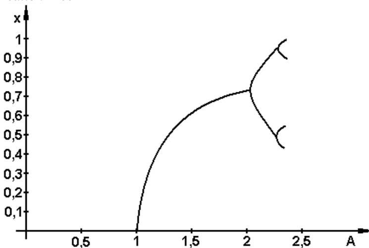
Figure 7: Bifurcation Tree
